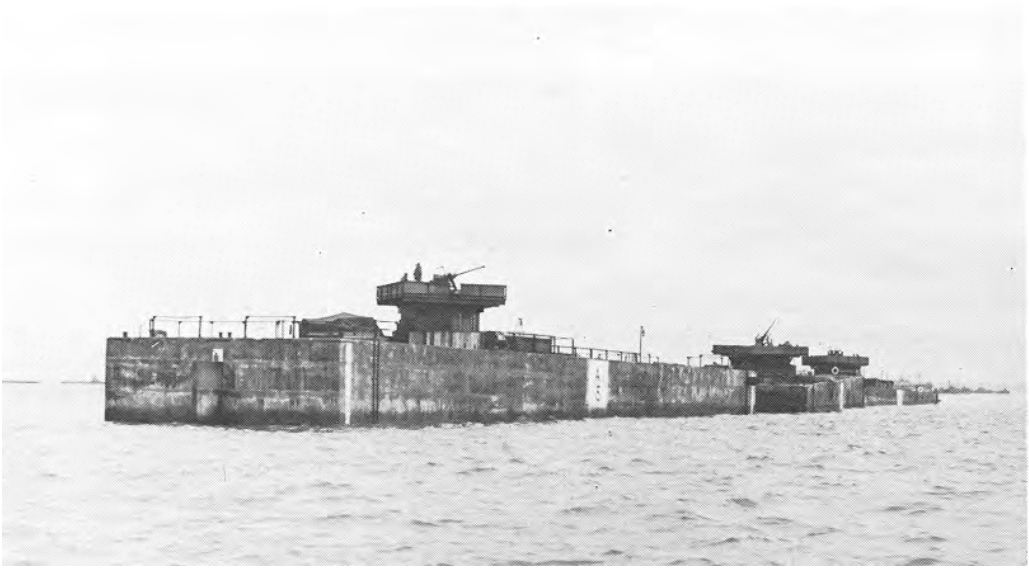
CAISSONS, used for MULBERRY breakwater, sunken in position off the beaches, above, and afloat, below.
